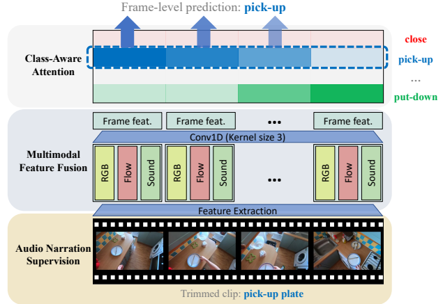
Figure 2. Model overview. We first cut the video into clips using the single timestamp denoted in the audio narration. Then, each video clip can be treated as a bag of a few actions. Next, we extract multimodal features and use early fusion to combine them (Sec. 3.1). We use a class-aware attention mechanism to produce the frame-level detection score (Sec. 3.2). Finally, we use a class-aware, intensity-sensitive post-processing (Sec. 3.3) to turn the frame-level into instance-level prediction (not shown), for evaluation purposes.
